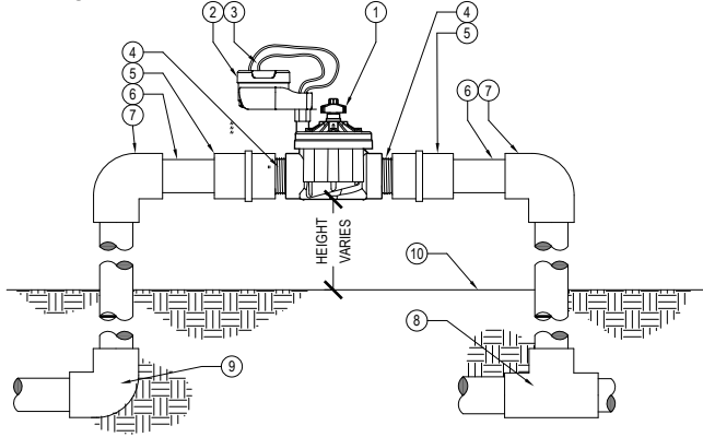
XX IN-LINE VALVE (ICV) WITH CONTROLLER (SENNODEBT) VC.ICV.1 NO SCALE
