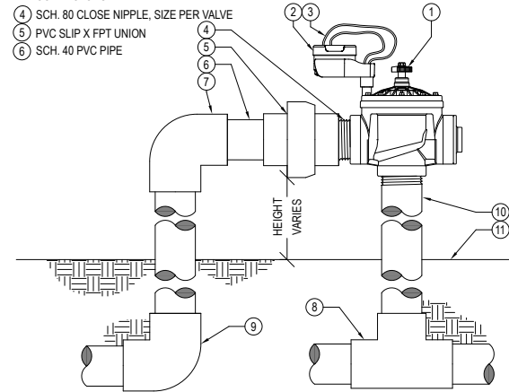
XX ANGLE VALVE (ICV) WITH CONTROLLER (SENNODEBT) AND UNION VC.ICV.4 NO SCALE
