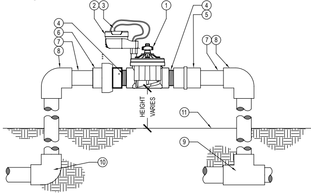
XX IN-LINE VALVE (ICV) WITH CONTROLLER (SENNODEBT) AND UNION VC.ICV.2 NO SCALE
