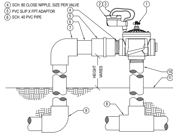
XX ANGLE VALVE (ICV) WITH CONTROLLER (SENNODEBT) VC.ICV.3 NO SCALE
