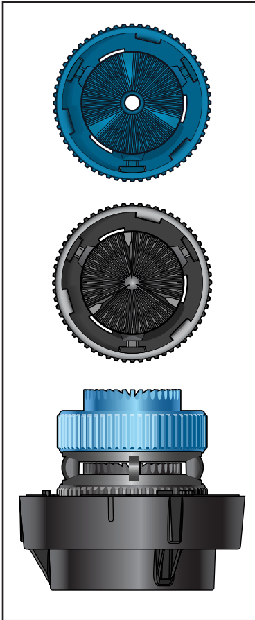
① LDNPHD2CFUP3B 2 = Double Pad C = Concave ( blue ) (33) with 0.198" hole F = Flat ( black ) (33) UP3B = UP3 Bubbler Pad Assembly Nozzles #15 - #26
