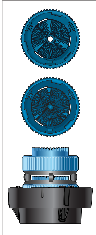
② LDNPHD2CCUP3B 2 = Double Pad C = Concave ( blue ) (33) with 0.198" hole C = Concave ( blue ) (33) UP3B = UP3 Bubbler Pad Assembly Nozzles #15 - #26
