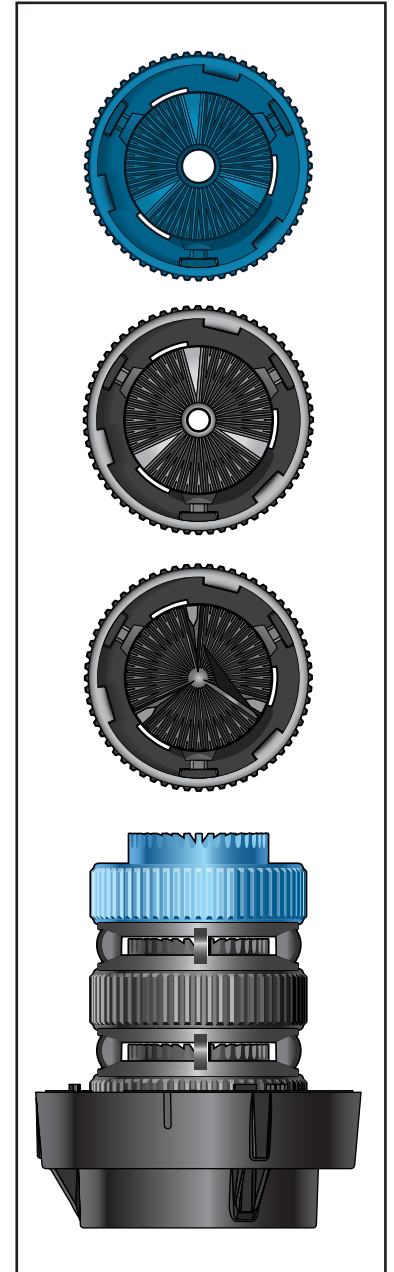
③ LDNPHD3CFFUP3B 3 = Triple Pad C = Concave ( blue ) (33) with 0.298" hole F = Flat ( black ) (33) with 0.198" hole F = Flat ( black ) (33) UP3B = UP3 Bub. Pad As'by Nozzles #20 - #26
